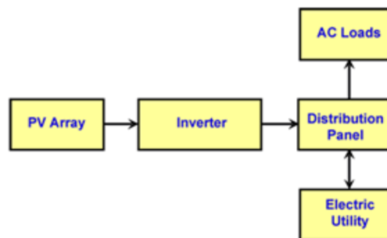
Figure 4. Simple interactive PV system.
