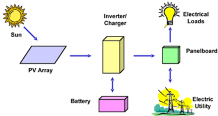
Figure 1. Solar photovoltaic (PV) system and typical components
