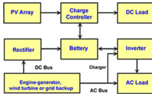
Figure 3. Stand-alone PV-hybrid system.
