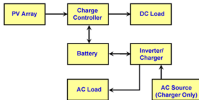
Figure 2. Stand-alone PV system with AC/DC loads.
